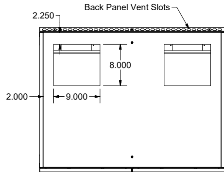
Top View Shown With Shelf
