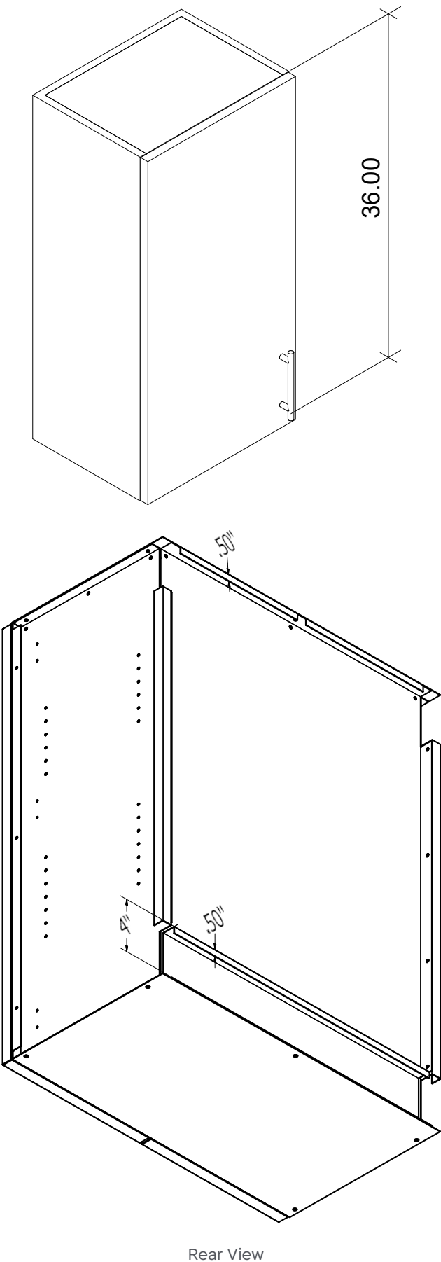
Rear View
