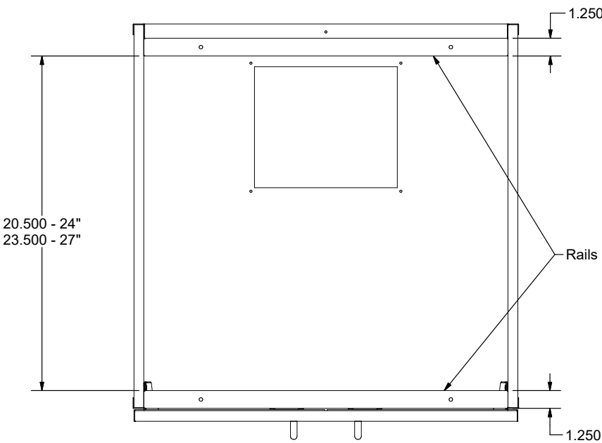
Plan View
